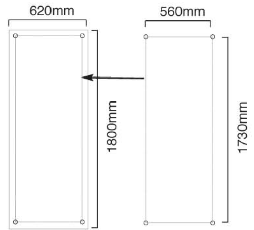
eyelet positioning 1730m (h) x 560mm (w) measuring to centrepoints of eyelets
