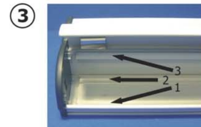
Lift open the lid and note the 3 grooves inside the base
